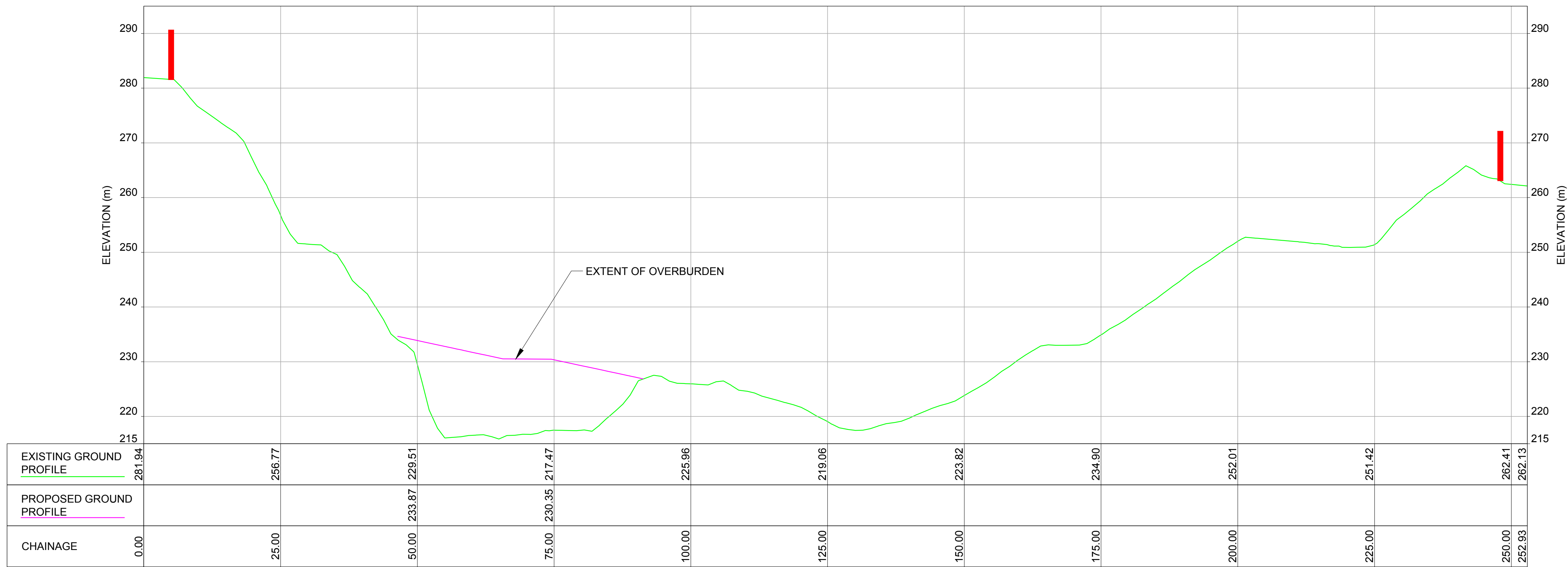
HOR. SCALE 1:500 m VERT. SCALE 1:500 m A 04 GROUND PROFILE
