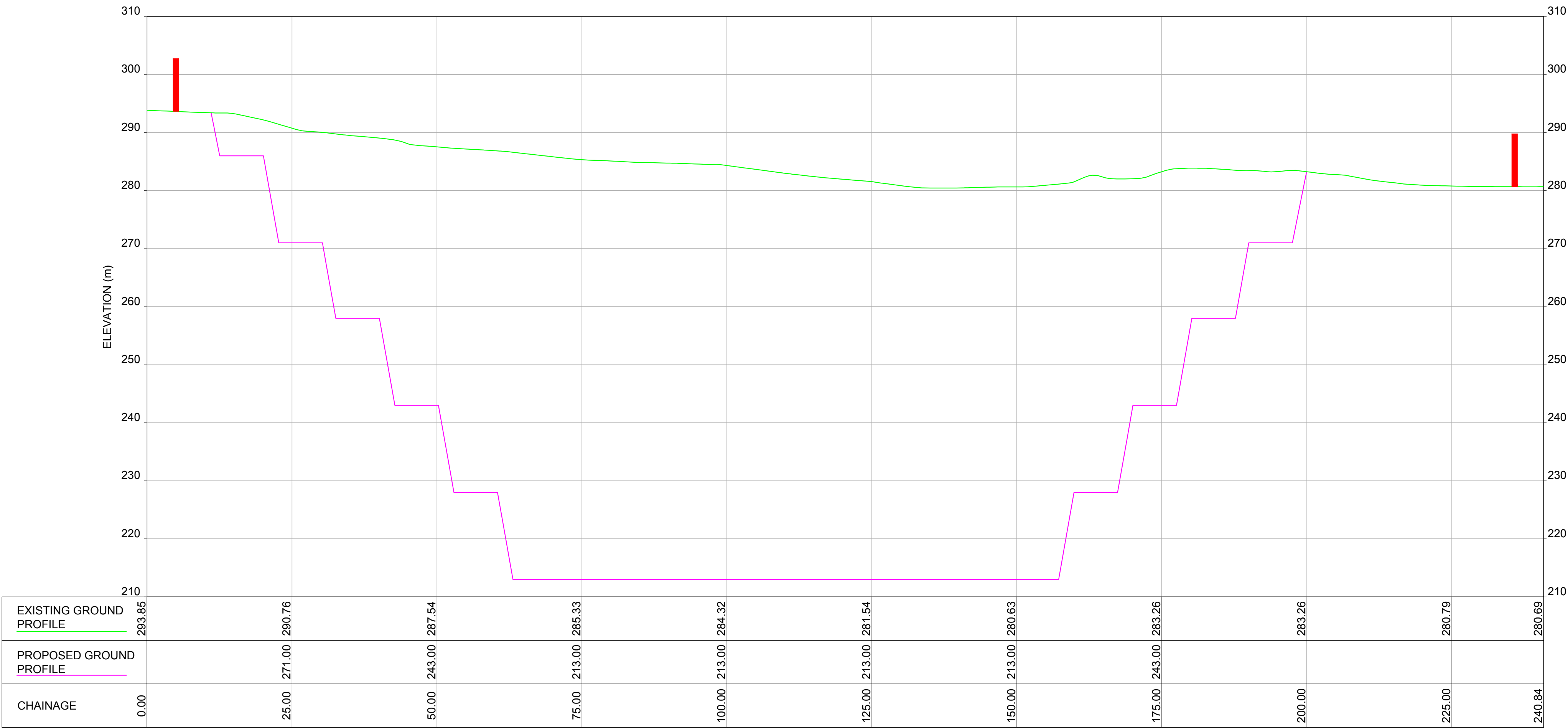
HOR. SCALE 1:500 m VERT. SCALE 1:500 m D 04 GROUND PROFILE
