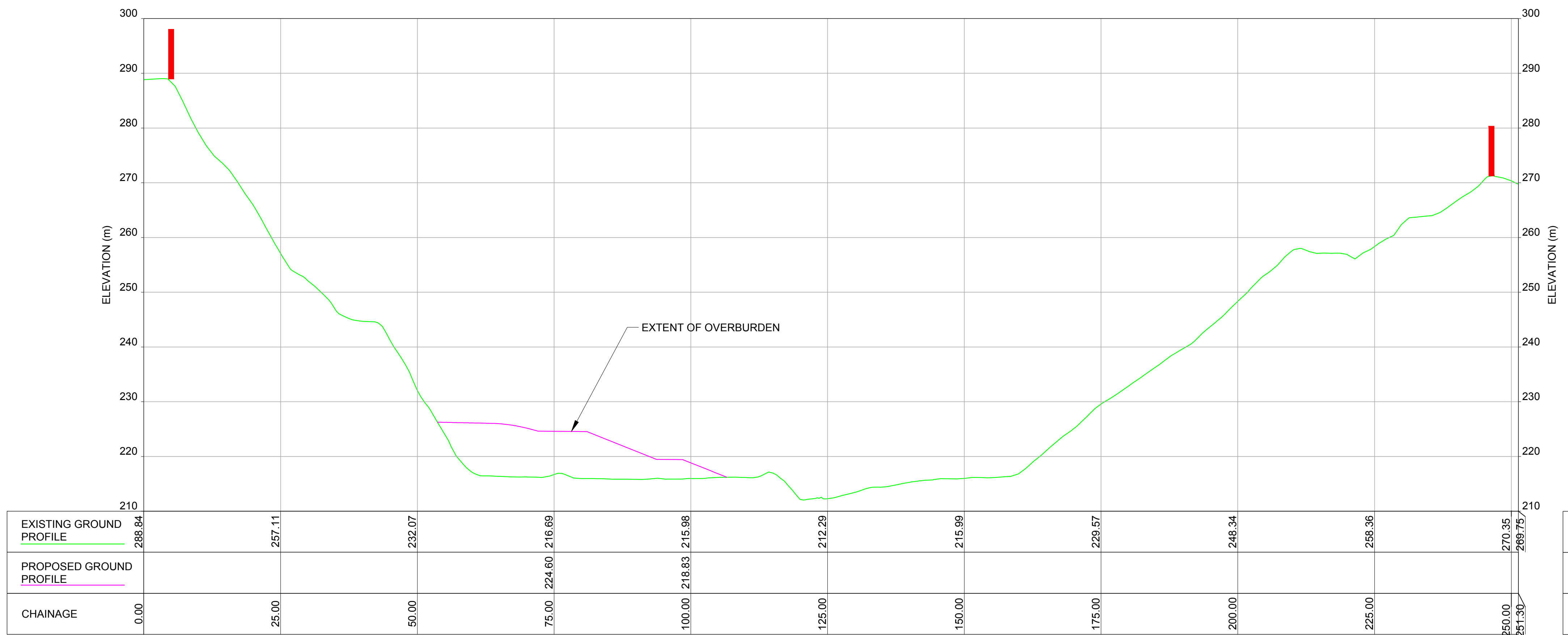
HOR. SCALE 1:500 m VERT. SCALE 1:500 m B 04 GROUND PROFILE
